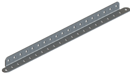
HANGAR LINK ARM - 1M / 3'3" Part No: LA1000
