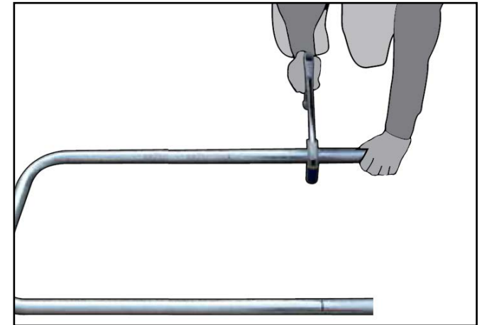
H. Using a hacksaw or similar carefully cut through the top and bottom tubes as shown. For galvanised assemblies, spray with Galvafoid or similar to prevent corrosion.
