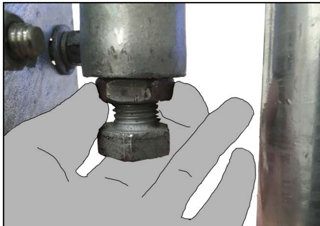
J. To tension the return spring hinge loosen the locking nut as shown.
