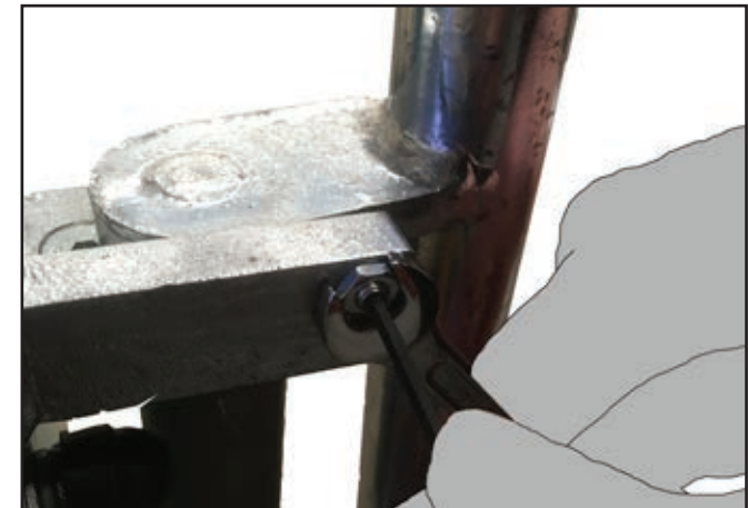
N. Using a M6 spanner and 4mm hex key, slacken off the locking nut and adjust the grub screws so that the gate leaves meet in the middle. Once centre position is correct, lock off grub screw using nut.
