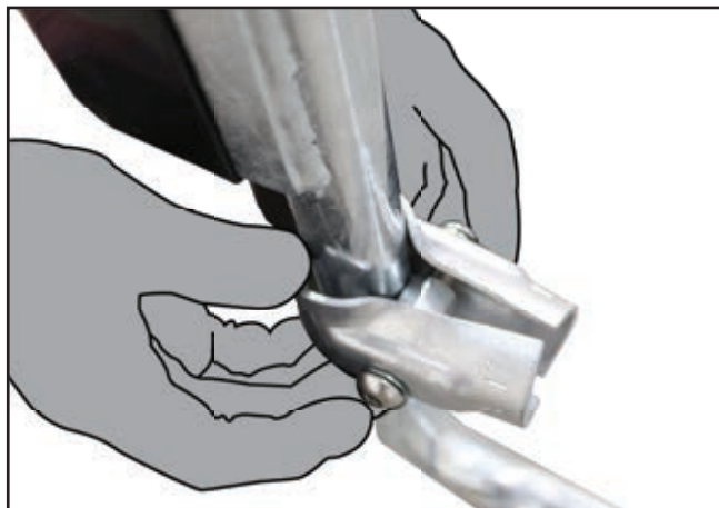
P. Mount clamp on lower part of gate, just above the bend and insert mid rail. Use 6mm hex head socket to tighten supplied M10 bolts into coupling nut.
