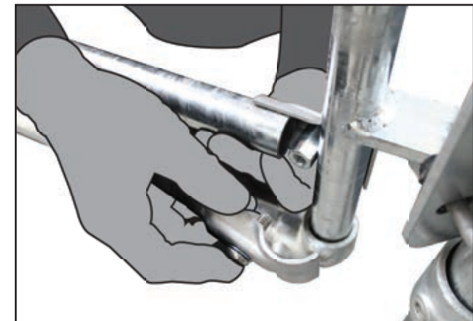
Q. Add clamp onto other end of mid rail, clamping onto the gate upright. Use 6mm hex head socket to tighten supplied M10 bolts into coupling nut.
