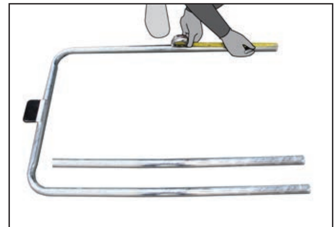
H. Divide the distance recorded in step F by 2, mark this measurement on gate top, bottom and mid rail tubes as shown.
